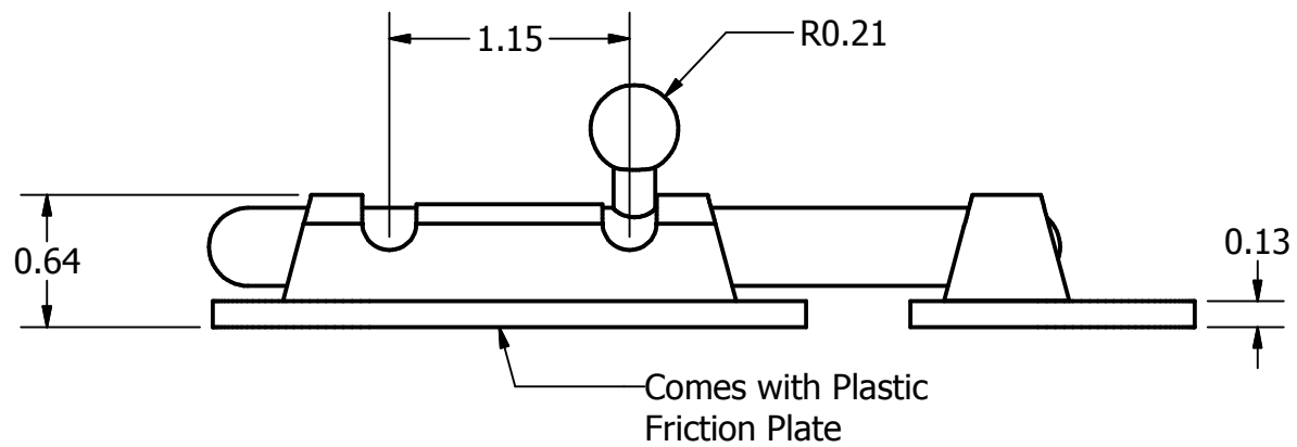
1455 Barrel Bolt
