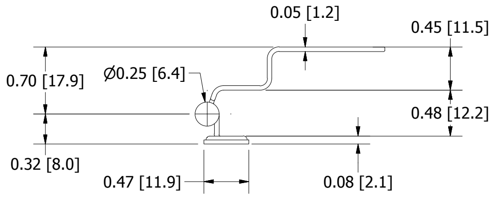
1653 2" x 1-1/2" Hinge, Offset
