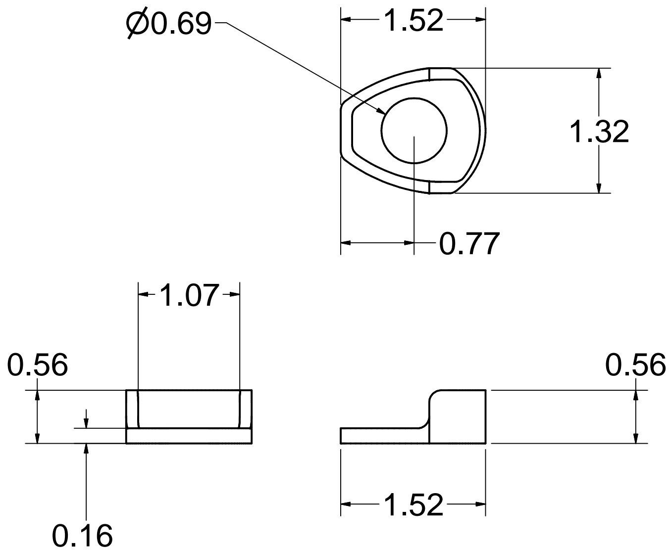
4498 Vent Cover
