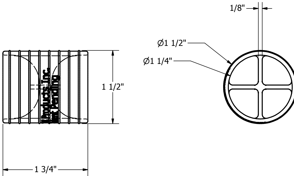
99900 1-1/2" Anti Fuel Theft Device
