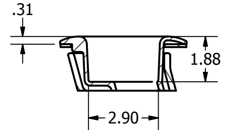
SECTION B-B CUP DIMENSIONS
