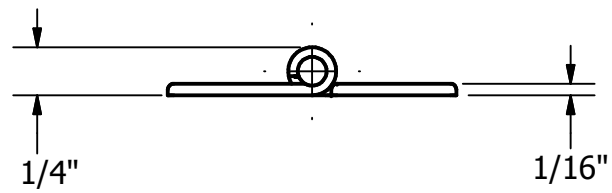
1224 1-1/2" x 2" Hinge, Coastal, Top Mount
