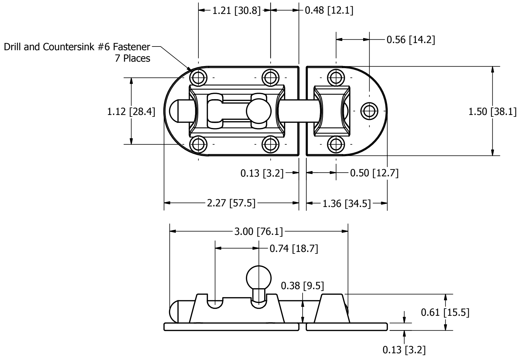
1454 Barrel Bolt
